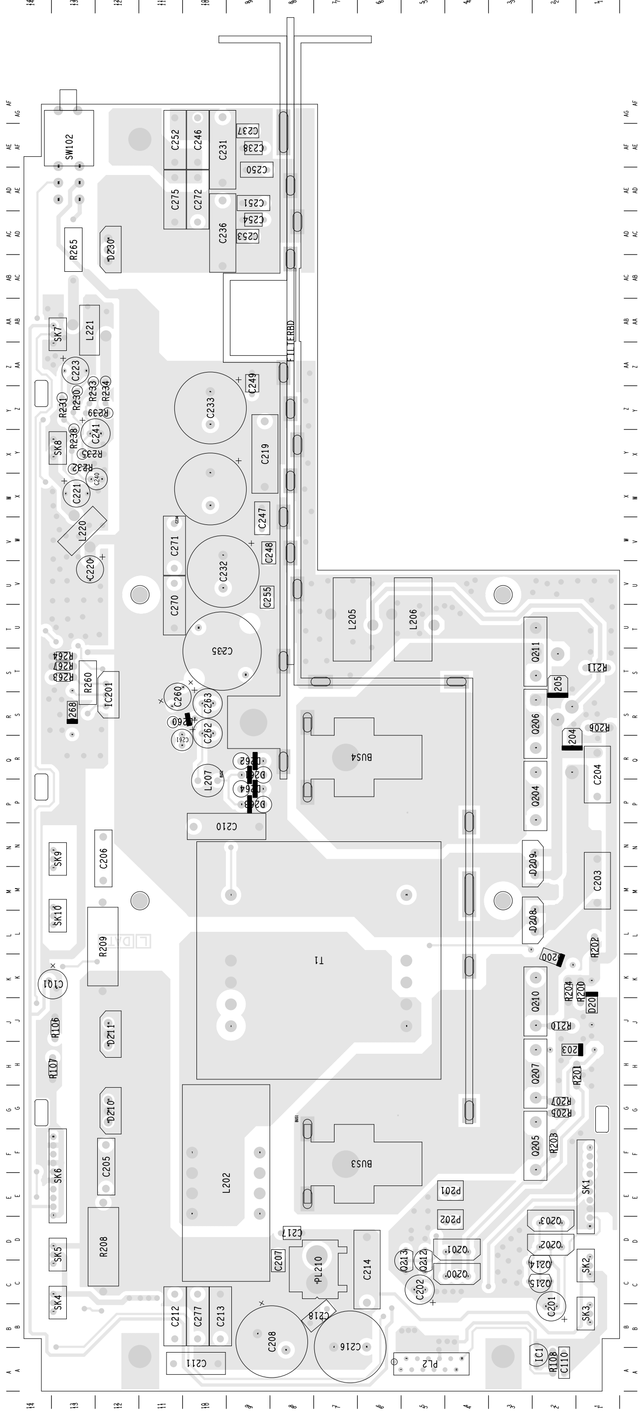
TAIT ELECTRONICS 220-02041-03 A 30Mx05 ANT TB8000 24V DC-DC CONVERTER LAYOUT-PRIMARY-SIDE
